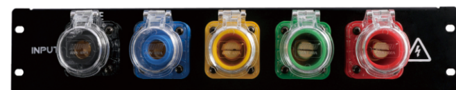
400A US Power Panel
