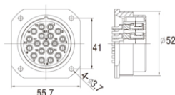
19-PIN MALE SOCKET 19芯公座
